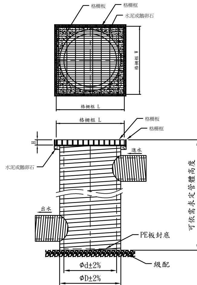
MHS30X, MHS40X, MHS60X, MHS80X陰井示意圖
